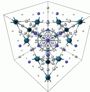
Al 10 V crystal structure
